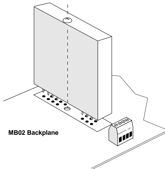
Figure 2-8. Mounting an MB Series Module
